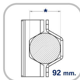
BPW – Ø 92
