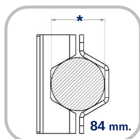
BPW – Ø 84
