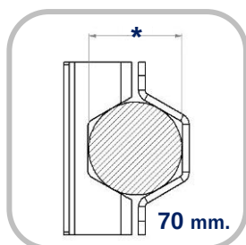
BPW – Ø 70
